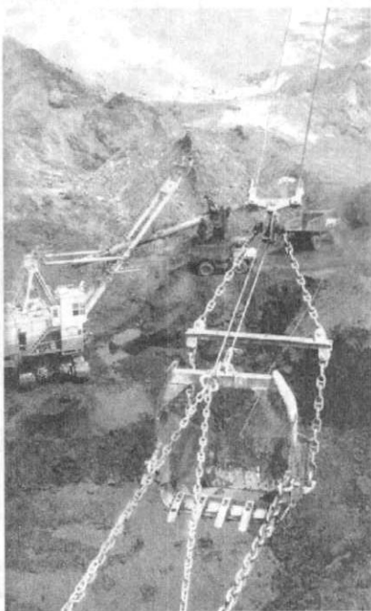
28-rasm. Angren ko'mir konida ko'mir qazib olish.
