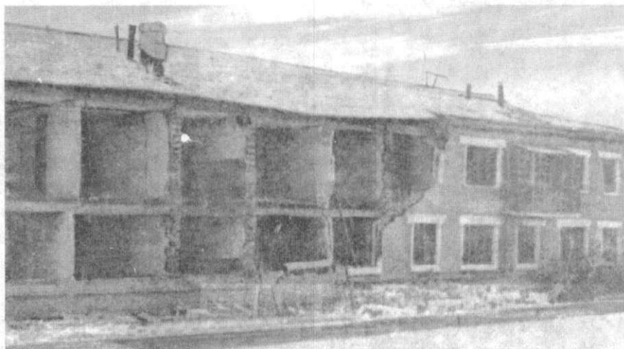
7-rasm. Gazli zilzilasida buzilgan bino (1976-y.)
