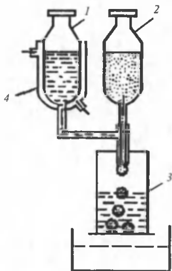
10-rasm. Tomchilab kapsula oladigan asbob.
