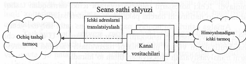
8.8-rasm. Seans sathi shlyuzining ishlash sxemasi.
