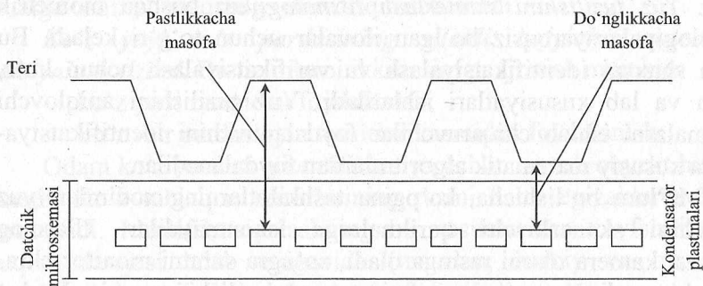
6.6-rasm. Sensor ishlashining prinsipi.
