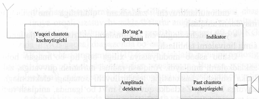
10.4-rasm. Elektromagnit nurlanish indikatorining sxemasi.
