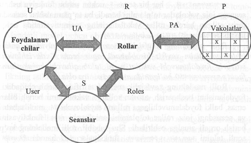
4.1-rasm. Foydalanishni boshqarishning roli modeli.
