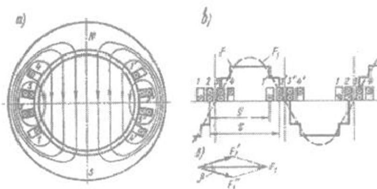
2.17-rasm. Ikki qutbli mashinaga oid ikki qatlamli qisqartirilgan qadamli stator chulg'amining qirqimi (a) va mazkur chulg'am MYK ning taqsimlanish diagrammasi (b)
