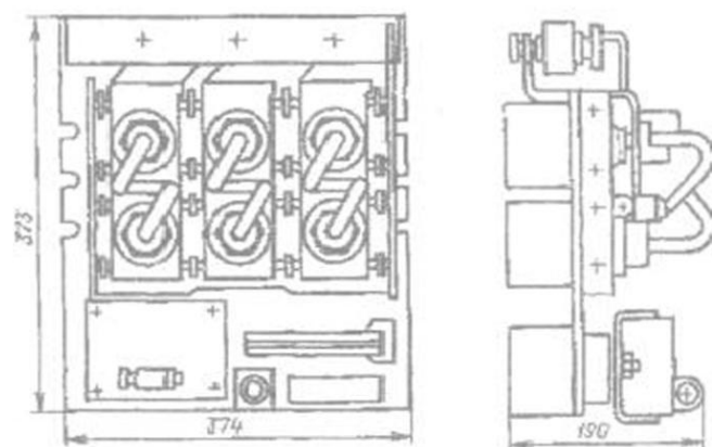
Rasm.7.11 . Tiristorli PT-40-380-U5 yuritkichi
