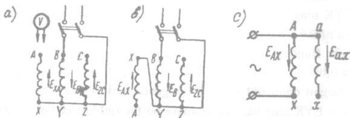
1.8-rasm. Transformatorning YK chulg'ami uchlari to'g'ri (a) va noto'g'ri (b) belgilangan uchun hamda chulg'am uchlari belgilanishini tajribada tekshirish uchun (c) sxemalar
