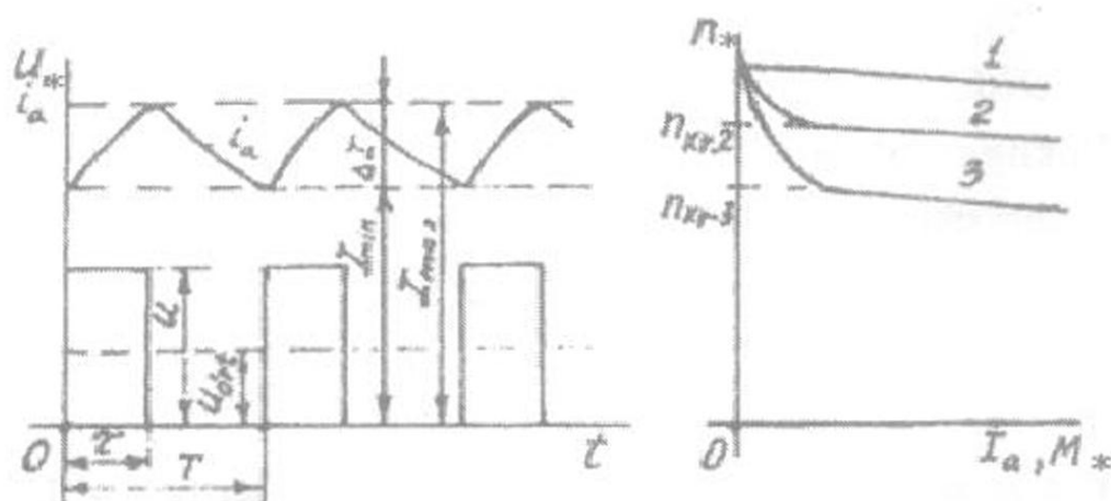
5.36-rasm. O'TM ning aylanish chastotasini impulsli rostdashda kuchlanish va toklarning o'zgarish grafigi (a) va parallel qo'zg'atishli motorni impulsli rostdashda tezlik va mexanik xarakteristikalar (b).
