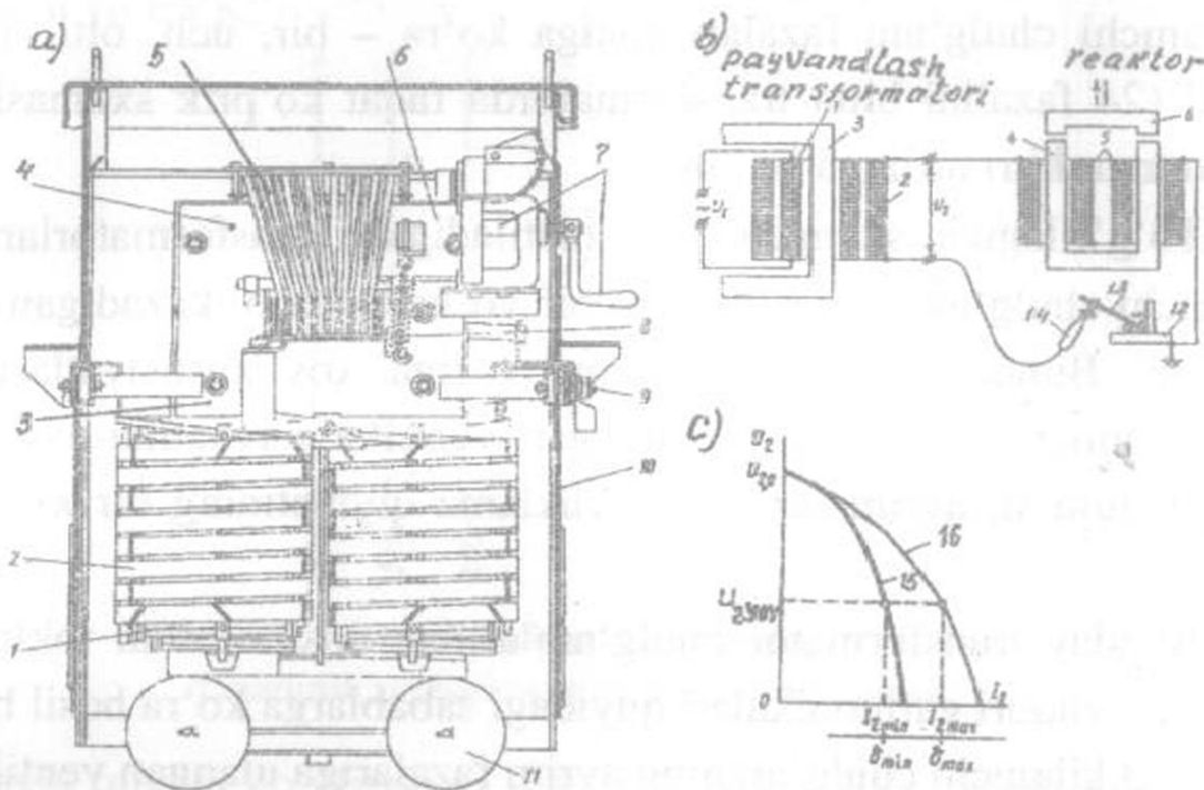
1.27-rasm. STN-500-1 tipli payvandlash transformatorining tuzilishi (a) va ishini prinsipial sxemasi (sxemada reaktor ajratib ko'rsatilgan) (b): [1, 2 – tegishli YK va PK chulg'amlar;
