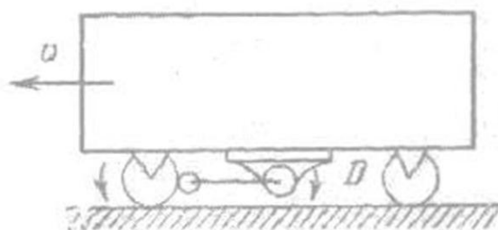
6.5-rasm. Transport mexanizmining gorizontaal harakatlanganda statik yuklamani hisoblashning prinsipial sxemasi.
