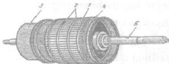
5.2-rasm. O'zgaras tok mashinasining yakori: 1 – yakor o'zagi; 2 – bandajlar; 3 – kollektor; 4 – yakor chulg'amining pazlardan tashqari qismi; 5 – o'q.
