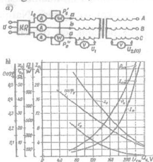
1.11-rasm. Quvvati S_N = 100 \text{ kV}\cdot\text{A} ; U_{1N}/U_{2N} = 6,3/0,22 \text{ kV} ; chulg'amlari Y/Y ulangan, uch fazali transformatorning salt ishlash tajribasini o'tkazish sxemasi (a) va salt ishlash xarakteristiklari (b); K.R – kuchlanishni rostlagich
