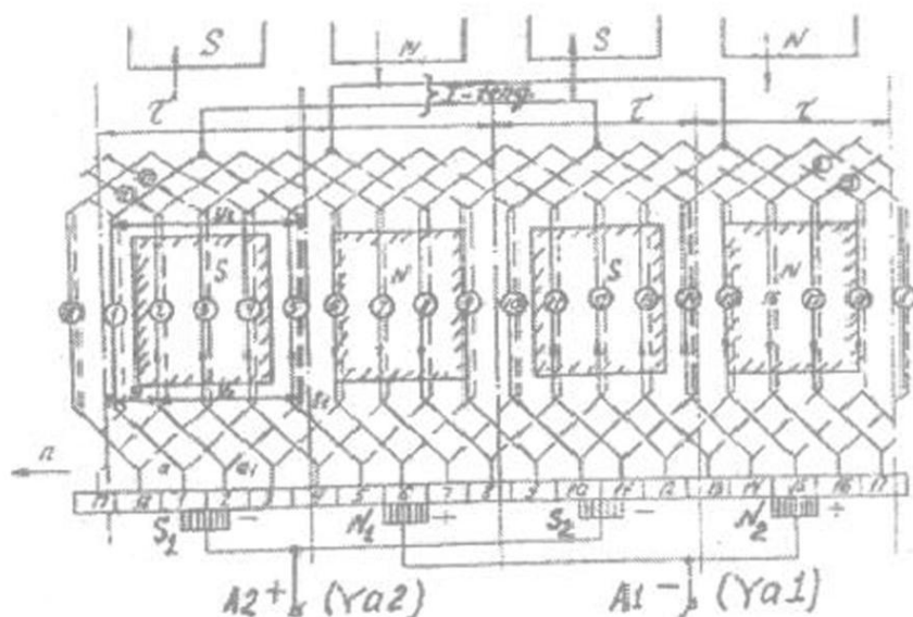
5.9-rasm. Oddiy o'ng yo'li sirtmoqsimon chulg'amning yoyilma sxemasi ( S = K = 18 , 2p = 4 , y_n = 1 ); I-teng – I_{tur} tenglashtirgichlar
