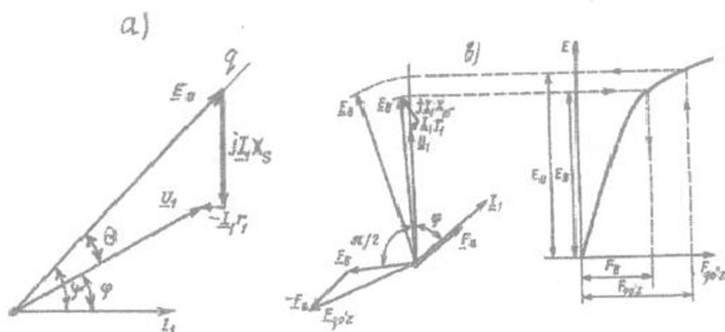
4.9-rasm. Ayon bo'lmagan qutbli SG ning aktiv-induktiv xarakterli yuklamadagi vektor diagrammalari: a – magnit zanjirining to'yinishi hisobga olinmagan hol uchun; b – magnit zanjirining to'yinish darajasi hisobga olingan hol uchun;
