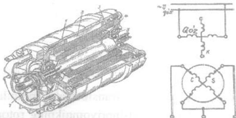
3.24-rasm. Aylanuvchi transformatorning umumiy ko'rinishi (a): 1 - korpus (tana), 2 - stator, 3 - stator chulg'ami, 4 - rotor, 5 - rotor chulg'ami, 6 - kontakt halqalar, 7 - cho'tkalar; b - prinsipial sxemasi
