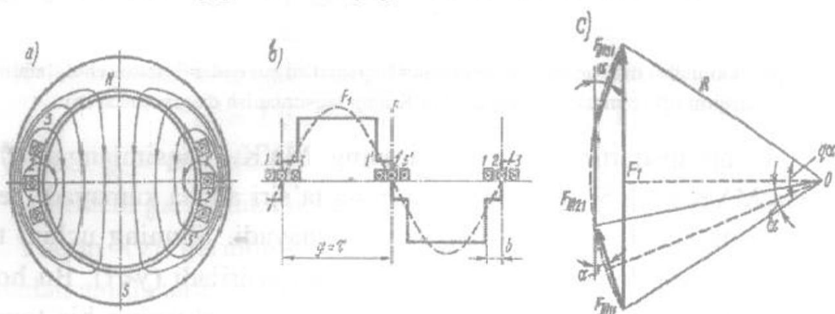
2.16-rasm. Ikki qutbli mashinaga oid ikki qatlamli taqsimlangan stator chulg'amining ko'ndalang qirg'imi (a), chulg'am MYK ning taqsimlanish diagrammasi (b) va stator pazlarida taqsimlangan g'altaklar MYK larining 1-garmonika vektorlarini qo'shish diagrammasi (c)
