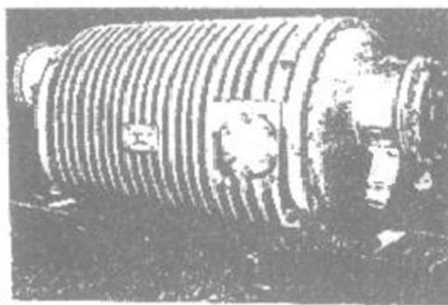
1.23-rasm. Quvvati 160 kVA, kuchlanishi 6 kV bo'lgan TSV-160/6 tipli portlashdan himoyalangan transformator.
